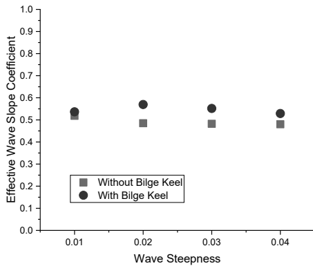
Figure 8: Effective wave slope coefficient
