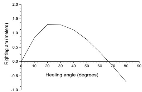
Figure 2: Righting arm curve of the subject ship
